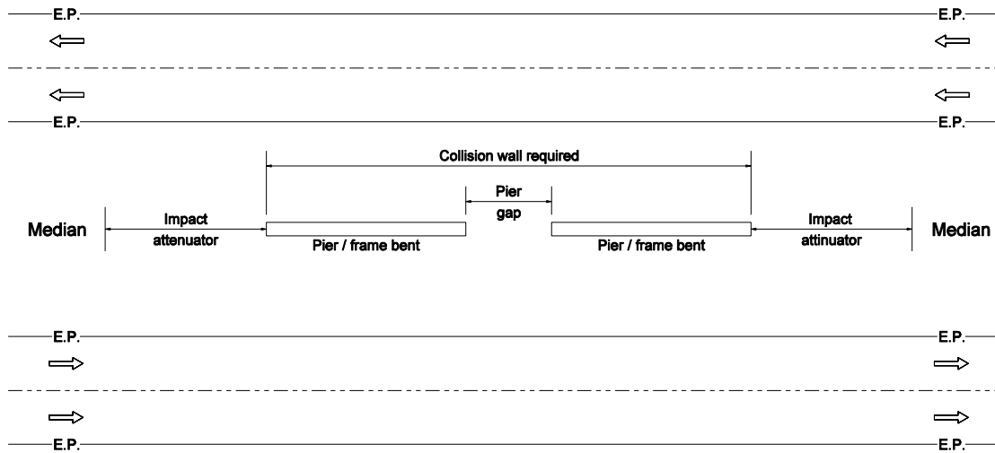
MULTI-LANE DIVIDED WITH TWIN OVERHEAD STRUCTURE AND MEDIAN PIERS
