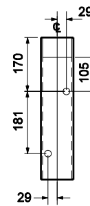
BACK VIEW
