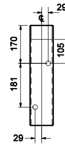
BACK VIEW
