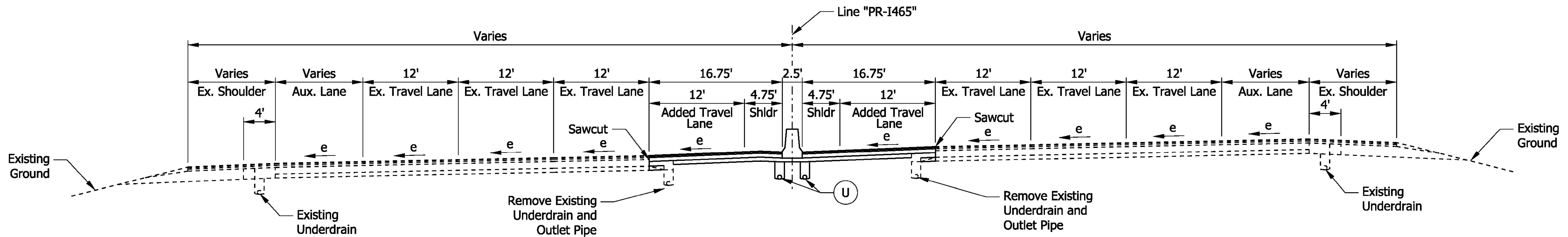
SUPERELEVATED TYPICAL SECTION PROJECT C
