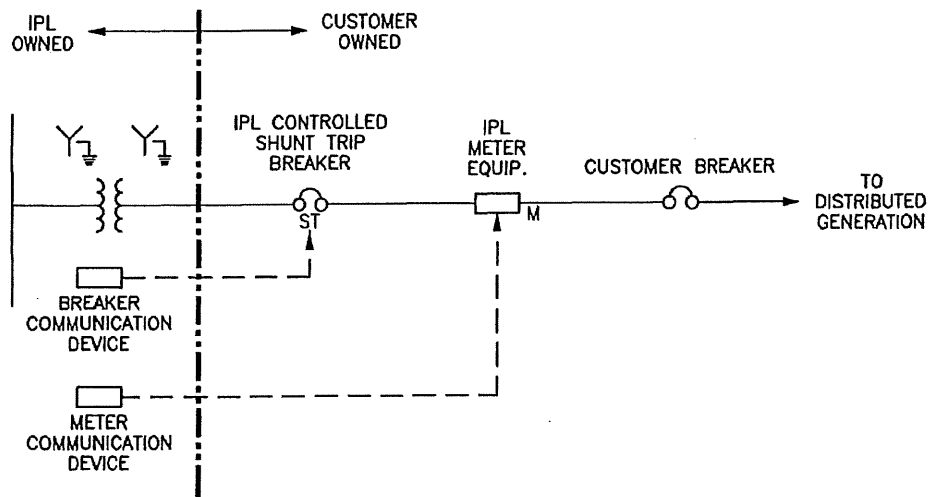
UNDERGROUND SINGLE LINE DIAGRAM
